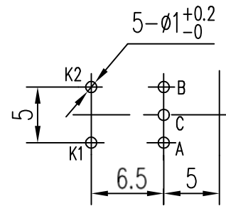
P.C.B MOUNTIONG HOLE DETAIL
