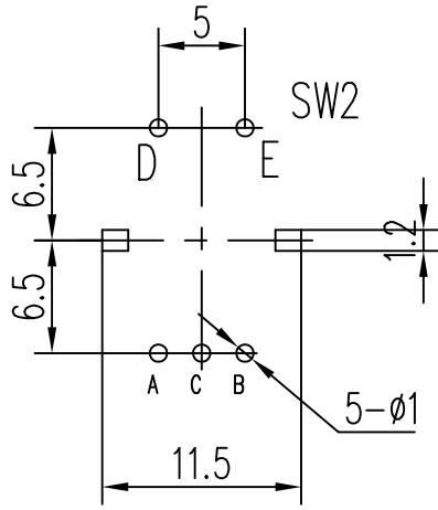
P.C.B MOUNTING HOLE DETAIL
