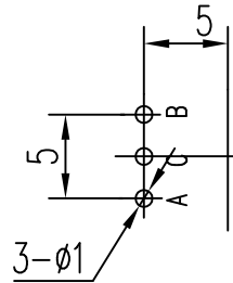
P.C.B MOUNTING HOLE DETAIL
