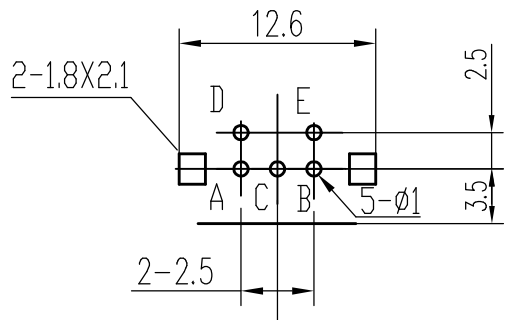
P.C.B MOUNTING HOLE DETAIL
