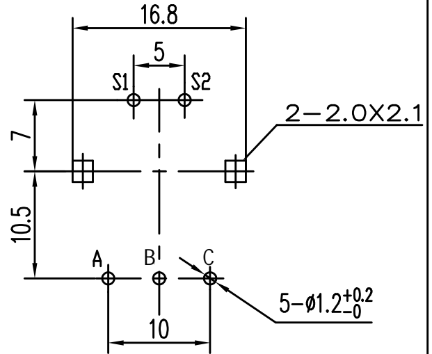
P.C.B MOUNTING DETAIL
