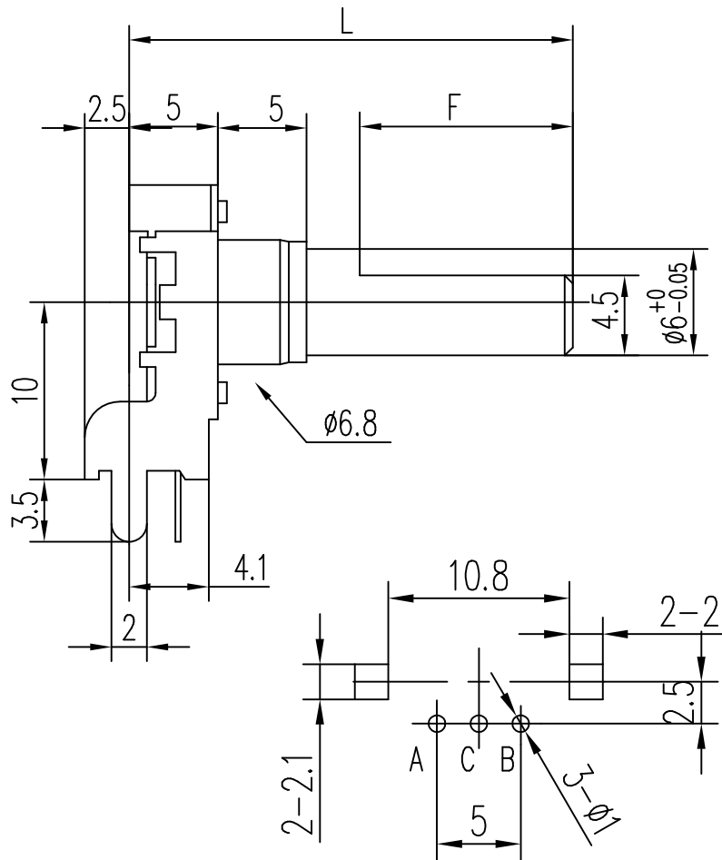
P.C.B MOUNTING HOLE DETAIL
